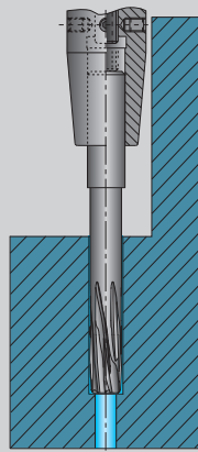
ALESATURA BORING
